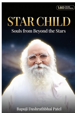
Star Child
